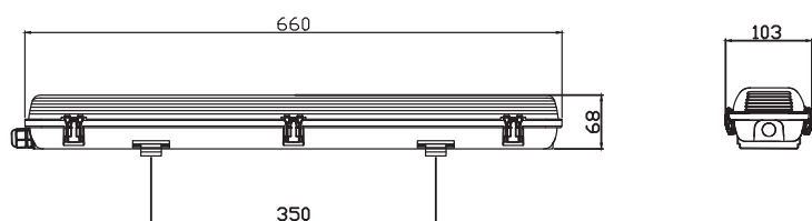
LED Waterproof Housing Poseidon V2.0 2x9W 600mm (2x18W eqv.)
