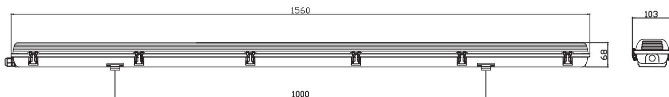
LED Waterproof Housing Poseidon V2.0 2x24W 1500mm (2x58W eqv.)
