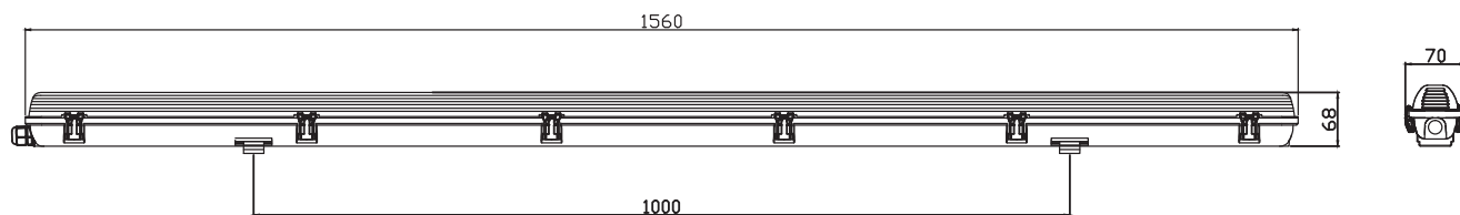
LED Waterproof Housing Poseidon V2.0 1x24W 1500mm (1x58W eqv.)
