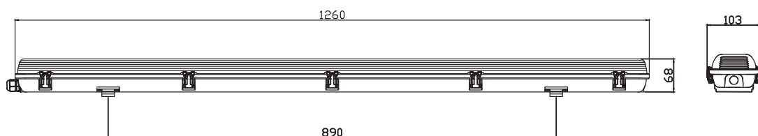
LED Waterproof Housing Poseidon V2.0 2x18W 1200mm (2x36W eqv.)
